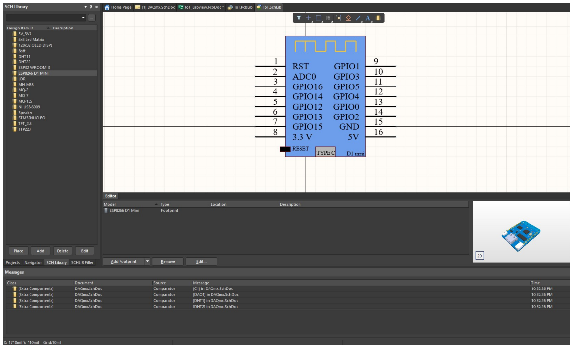
Crearea componentelor logic, Altium Designer 2026
